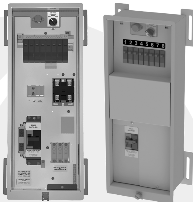
Front View (Lid and Cover Removed)
