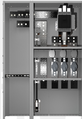
Front View Covers Removed
