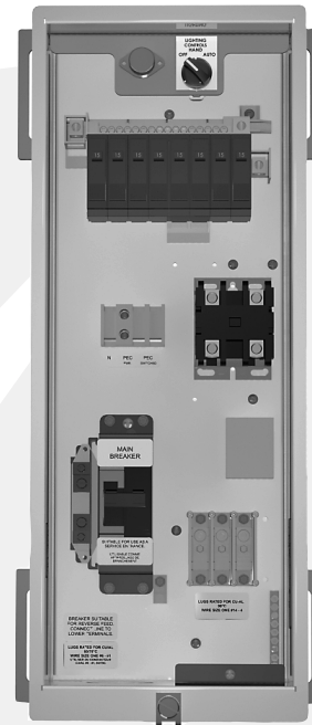
Front View (Lid and Cover Removed)
