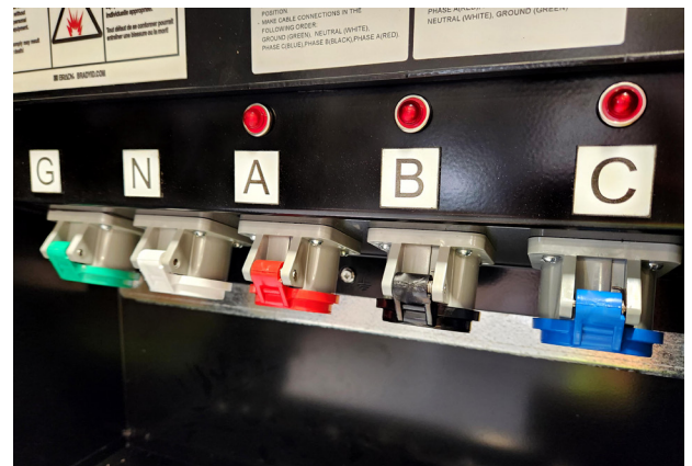
▲ Cam-Lock Connections
