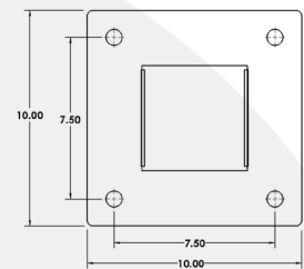
Standard Base
