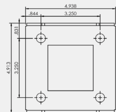
Hidden Base
