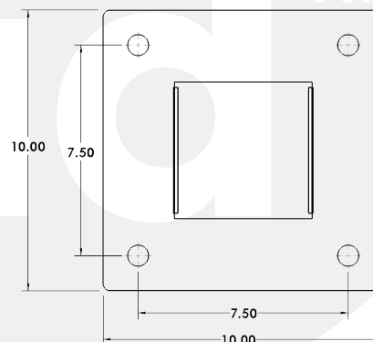
Standard Base Dimensions
