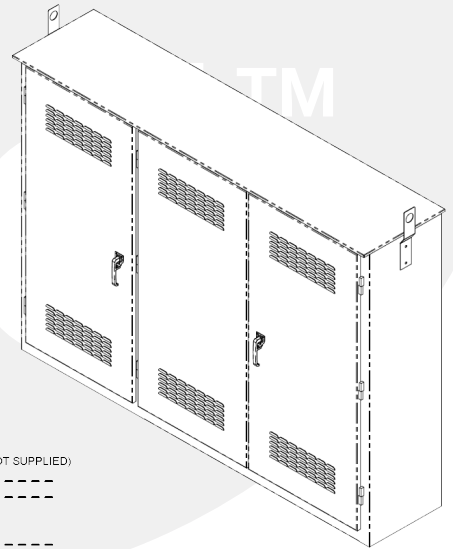
Typical FDC6 with MLO Breaker Panel Option
