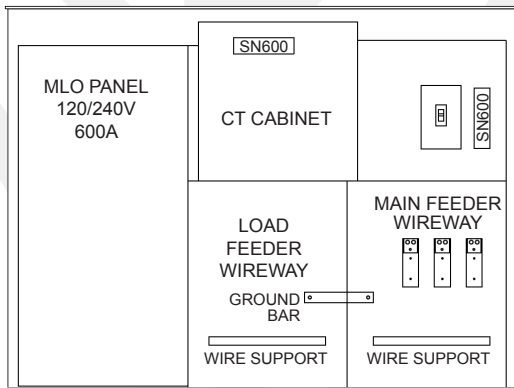
Typical FDC6 with MLO Breaker Panel Option
