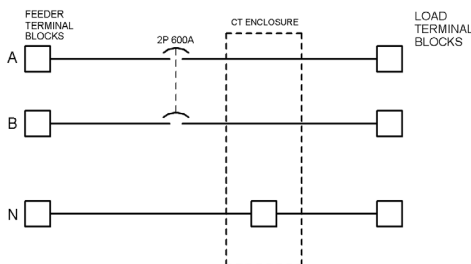
BUSSING OPTION - PRE-DRILLED AND TAPPED BUS CONNECTION FOR CT'S
