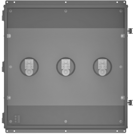
Front View (Door hidden, shown with polycarbonate cover)
