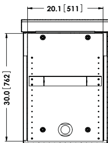
SECTION C-C (BACK PANEL DETAIL)
