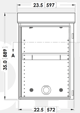
Front View (Door Removed)
