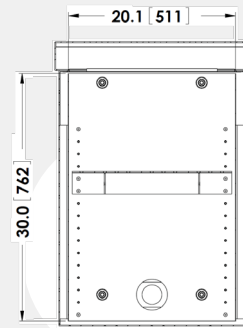
Back Panel Detail
