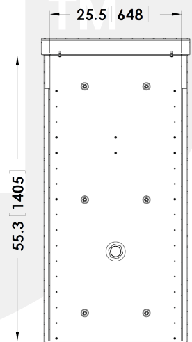
Section B-B Back Panel Detail
