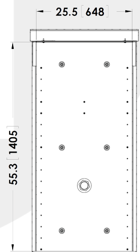
Section B-B Back Panel Detail
