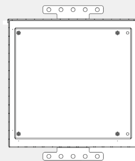
Section B-B Back Panel Detail
