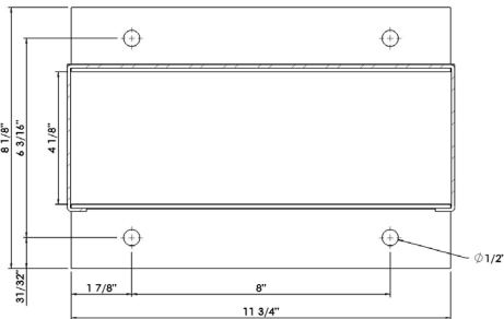
STANDARD BASEPLATE DIMENSIONS
