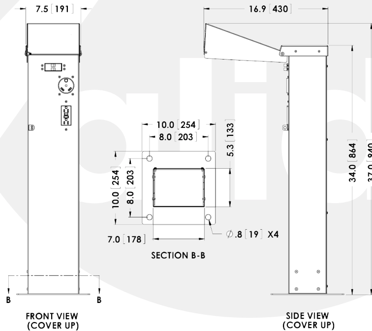
TYPICAL RVP3 CONFIGURATION
