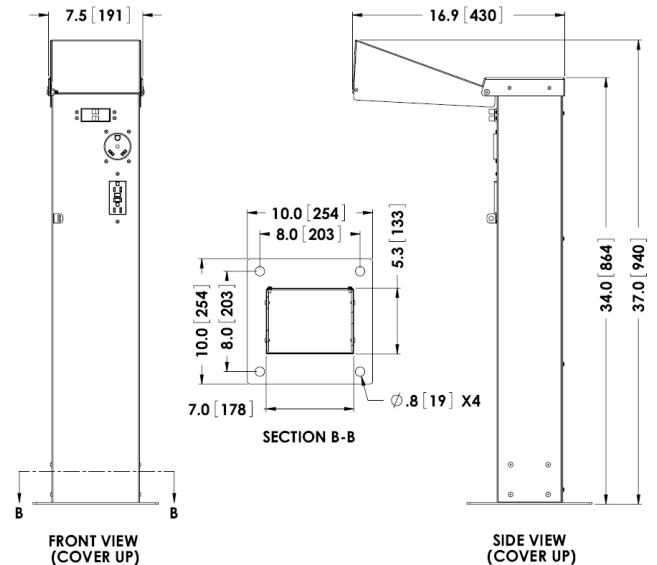
TYPICAL RVP3 CONFIGURATION
