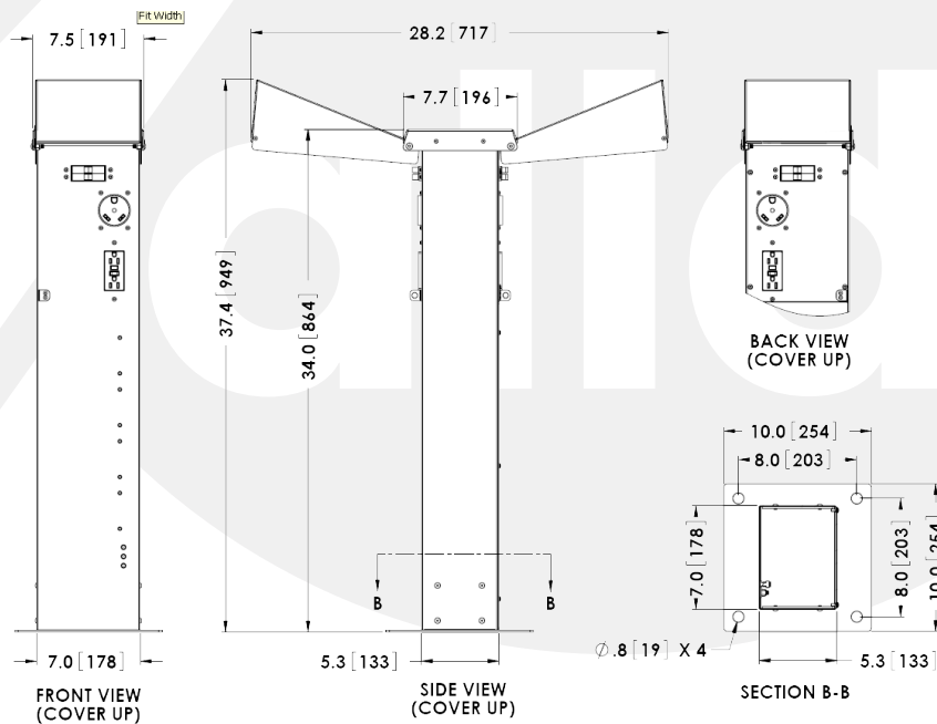
TYPICAL RVPD3 CONFIGURATION
