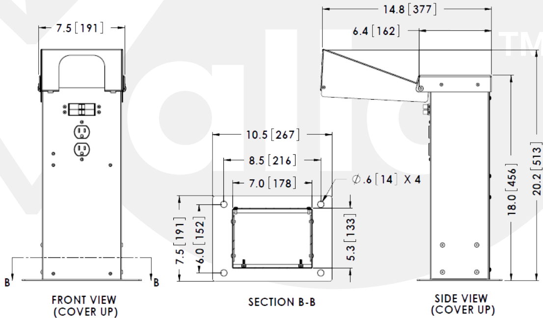
TYPICAL RVS CONFIGURATION
