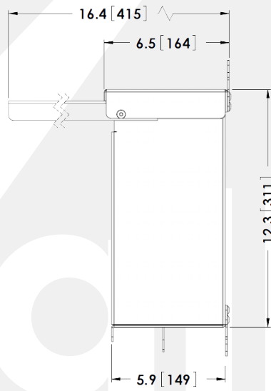
SIDE VIEW (COVER UP)
