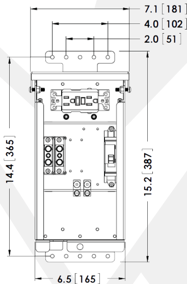
FRONT VIEW (COVER UP) (INTERIOR COVER REMOVED)
