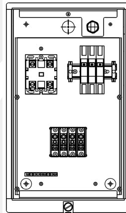
Lighting Controller Front View (Cover Off)
