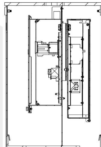
Sectional View of Complete Unit
