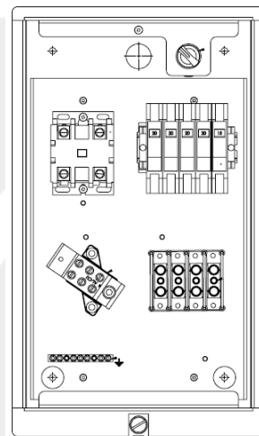
Lighting Controller Front View (Cover Off)
