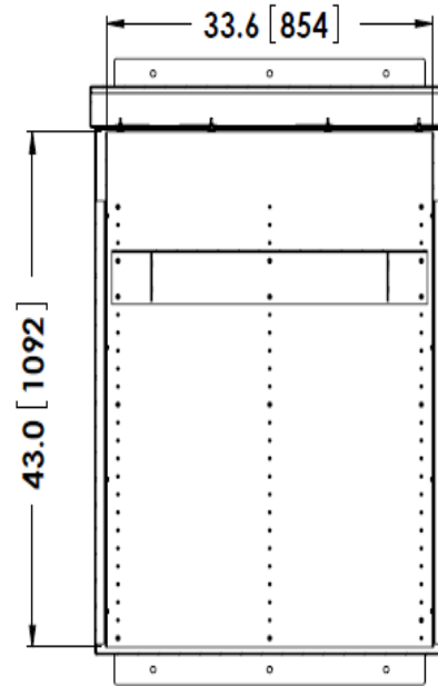
SECTION B-B (BACK PANEL)
