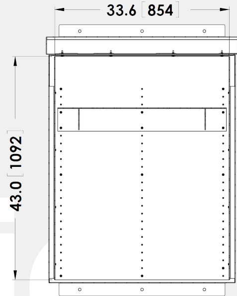
Section B-B (Back Panel)
