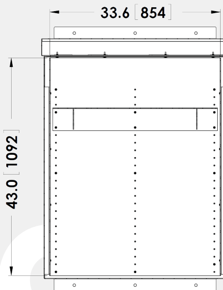
Section B-B (Back Panel)
